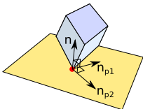
Figure : Friction collision basis
