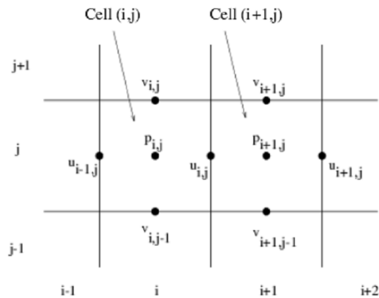
Figure 3: Staggered Grid for u , v , and p .
