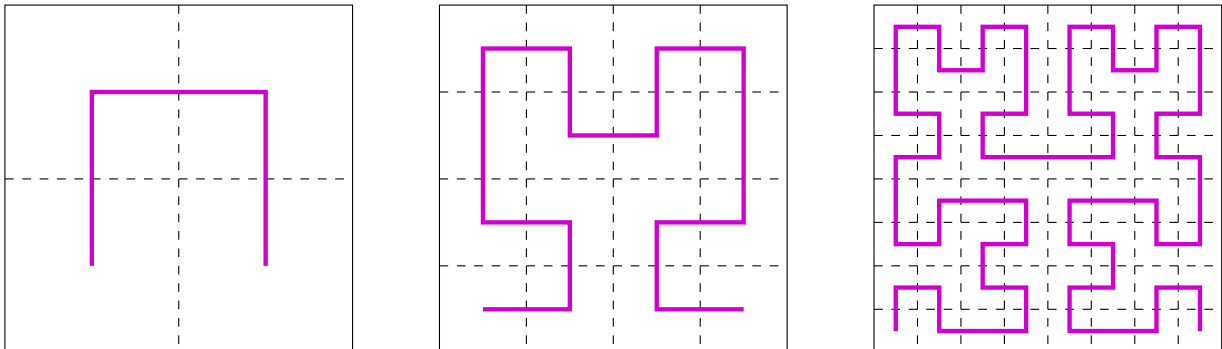
Abbildung 2: Construction of the Hilbert Curve
