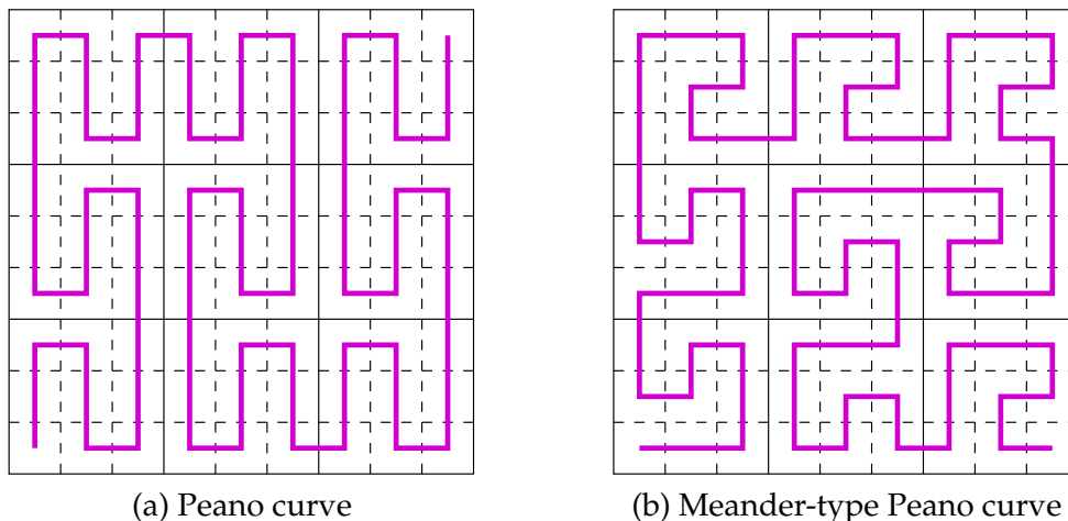
Abbildung 1: Two Peano-style space filling curves
