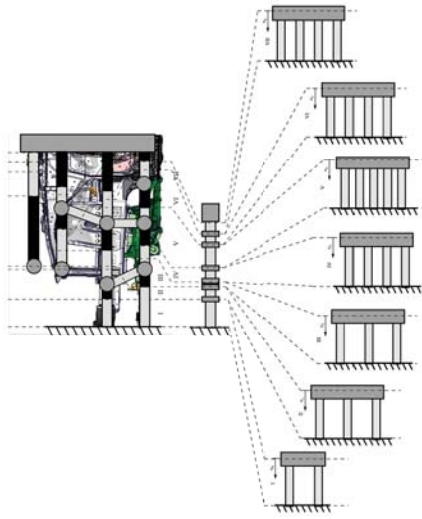
Figure 2: Decomposition of the system into load paths and components, Fender (2014) 2
