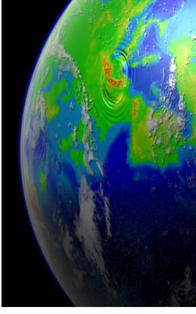
Project B2, result with SEISSOL: Visualisation of the propagation of seismic waves after an earthquake event in Central Europe after 100 seconds of propagation time. The faster P-waves have relatively low amplitudes compared to the slower S- and surface waves, which typically have higher damage potential
